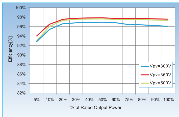
Efficiency Curve
